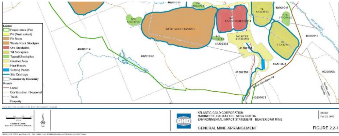
Beaver Dam Gold Project revised infrastructure layout
